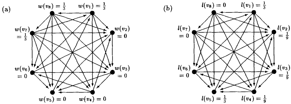
FIGURE 3. A Winning and Losing Density. This shows two densities on the tournament in Figure 1. Density w is winning because the inset of any node is at least as likely as its outset. For example, a node picked from this density will beat v_5 with probability 2/3 and will lose with probability 1/3 . Density l is losing because the outset of any node is at least as likely as its inset.
