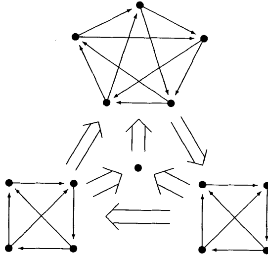
FIGURE 2. An Example. The center node in this tournament has outdegree five, while all other nodes have outdegree at least six. However the center node beats only nine nodes in T^2 . Thus, it not always true that a node of minimum outdegree beats at least twice as many nodes in T^2 as it beats in T (adapted from [1]).
