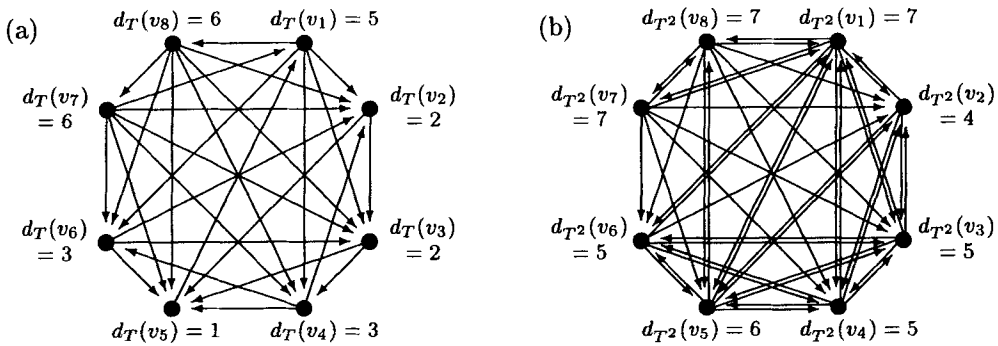
FIGURE 1. A tournament and its square. The labels show the outdegree of each node. Dean conjectured that any tournament has a node whose outdegree at least doubles in its square. Here there are three such nodes: v_2, v_3 , and v_5 .
